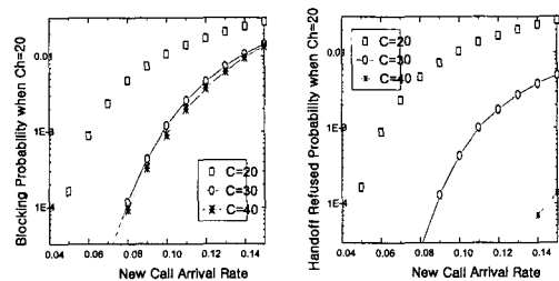
Fig 8. Proposed Scheme in the non-SDS System: Blocking and Handoff Refused Probability vs. New Call Arrival Rate with varying C
