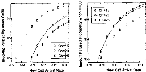
Fig 7. Proposed Scheme in the non-SDS System: Blocking and Handoff Refused Probability vs. New Call Arrival Rate with varying C_h
