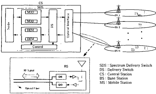
Fig 1. Fiber-Optic Cellular Radio System using SDS
