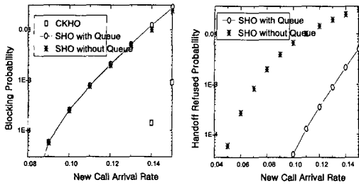
Fig 6. Comparison of Soft Handoff Scheme and Proposed Scheme in the SDS System: Blocking and Handoff Refused Probability vs. New Call Arrival Rate
