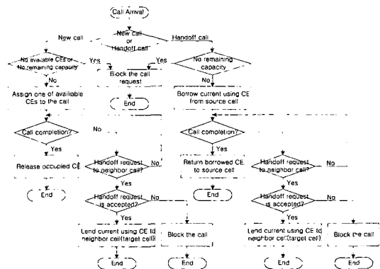
Fig 2. Proposed Handoff Algorithm
