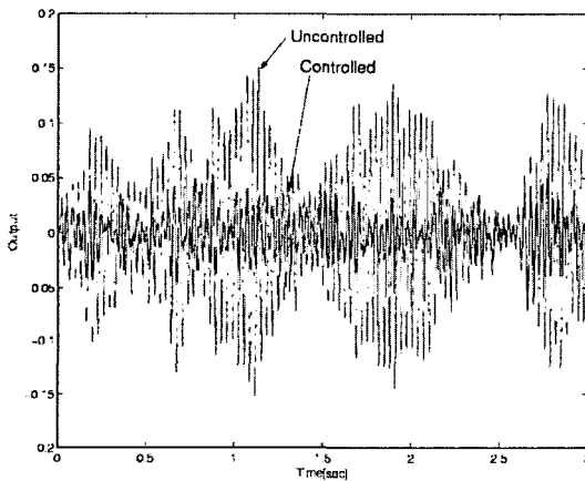
Fig. 6 Output system responses subject to random excitation
