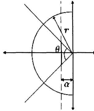
Fig. 3 Pole placement region
