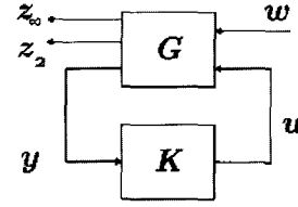
Fig. 2 Standard H_2/H_{\infty} feedback configuration
