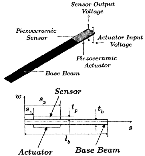
Fig. 1 Schematic drawings of smart structural system
