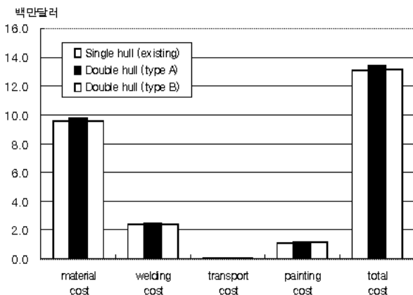
Fig. 3 Comparison of the construction cost
