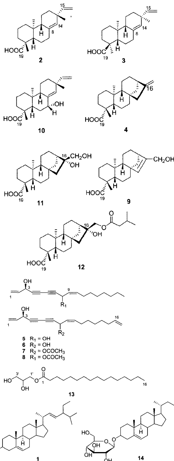
Fig. 1. The structures of compounds isolated from Aralia cordata
