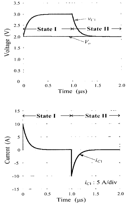
Fig. 5 Simulated key waveforms for conventional SCC. Conditions: I_o = 1\text{A} , r (= r_{S1} = r_{S2} = r_{S3} = r_{S4}) = 50\text{m}\Omega . (Half buck type)
