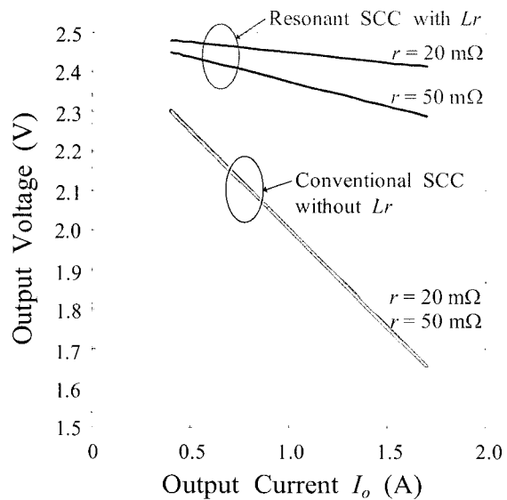
(b) Output current characteristics of output voltage
