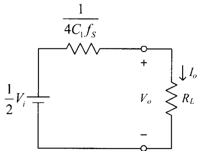
(a) Conventional SCC
