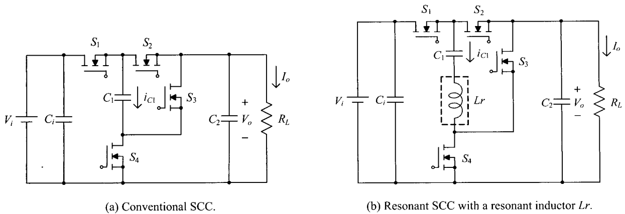
Fig. 9 Experimental circuits of the half buck type SCC's
