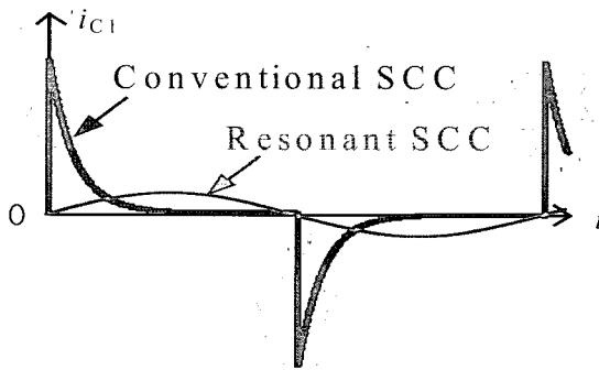
Fig. 2 Comparison of waveforms of the capacitor current between conventional and resonant SCC's. A large pulse current flows through C_1 in the conventional SCC, which brings about an inherent power loss at the internal resistance
