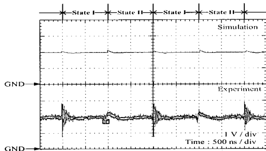
(b) Output voltage V_o
