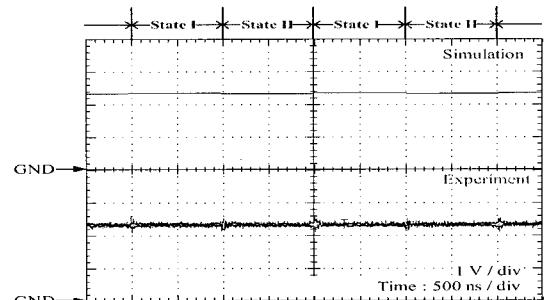
(b) Output voltage V_o
