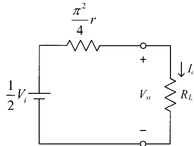
(b) Resonant SCC with a resonant inductor Lr .
