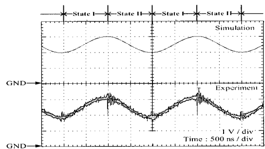
(a) Capacitor voltage v_{c1}
