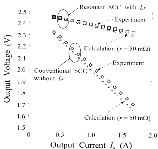
(b) Output current characteristics of output voltage
