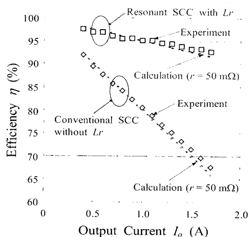
(a) Output current characteristics of efficiency
