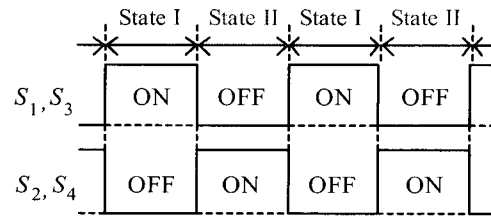
Fig. 3 Switching sequence for resonant SCC (Duty ratio = 50%)
