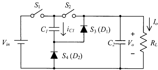
(a) Conventional SCC
