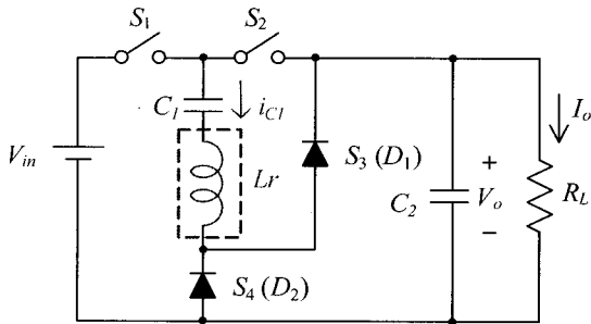
(b) Resonant SCC with a resonant inductor L_r
