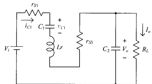
(a) State I
