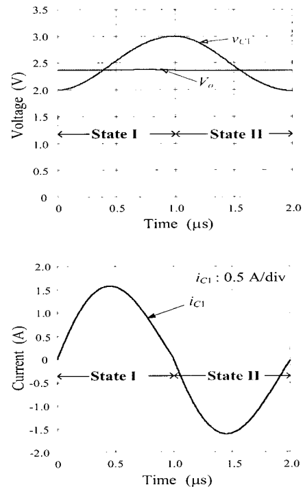
Fig. 6 Simulated key waveforms for Resonant SCC Conditions: I_o = 1\text{A} , r (= r_{S1} = r_{S2} = r_{S3} = r_{S4}) = 50\text{m}\Omega . (Half buck type)
