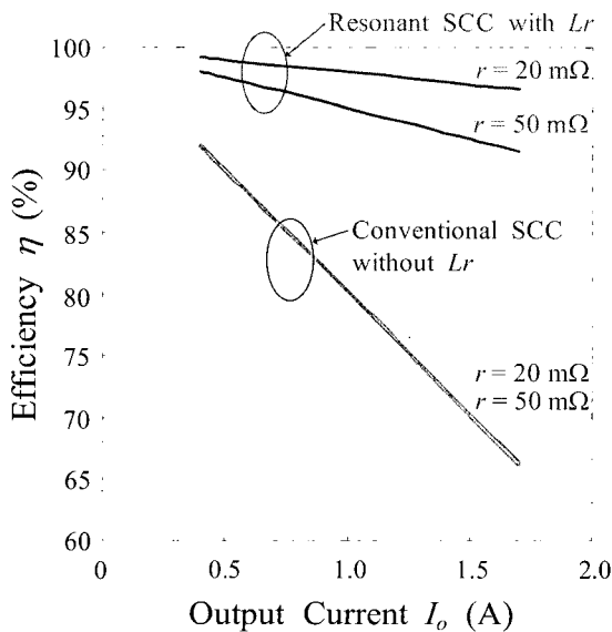
(a) Output current characteristics of efficiency
