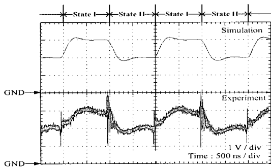
(a) Capacitor voltage v_{c1}
