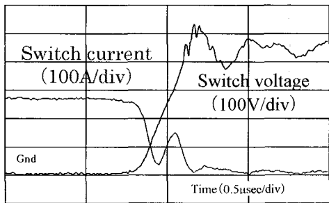
(b) Turn-off
