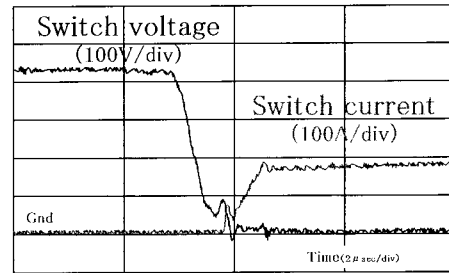
(a) Turn-on
