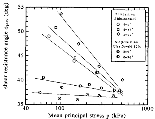
Fig. 12. Relationship between shear resistance angles at peak shear and mean principal stress
