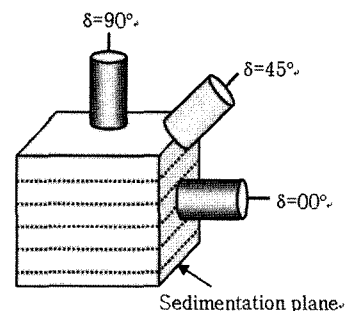
Fig 2. Schematic diagram of the sedimentation angle
