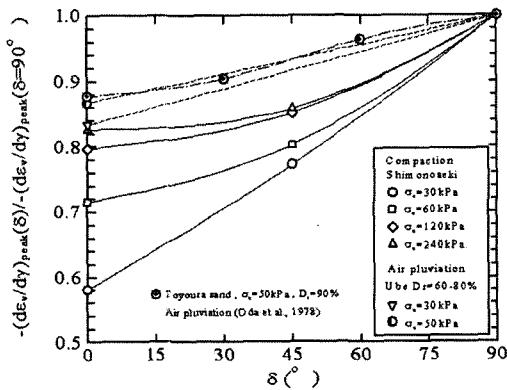
Fig. 13. -(d\varepsilon_v/d\gamma)_{peak}(\delta) / -(d\varepsilon_v/d\gamma)_{peak}(\delta=90^\circ) and \delta Relations
