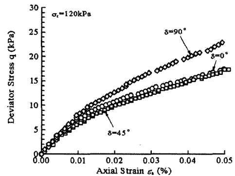
Fig 8. Stress-Strain relations ( \epsilon_a=0.05\% )
