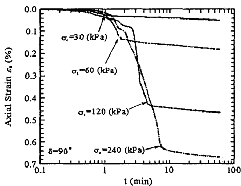
Fig 5. Relation between axial strain and compression
