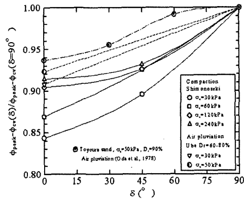
Fig. 14. \phi_{peak}-\phi_{cv}(\delta) / \phi_{peak}-\phi_{cv}(\delta=90^\circ) and \delta Relations
