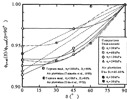
Fig. 11. Relationship between \phi(\delta)/\phi(\delta=90^\circ) and \delta
