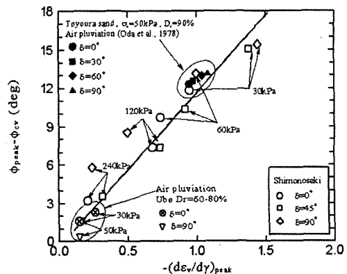
Fig. 15. Relationship between (\phi_{peak}-\phi_{cv}) and -(d\varepsilon_v/d\gamma)_{peak}
