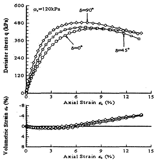
Fig 7. Stress-Strain relations with variations of sedimentation angle
