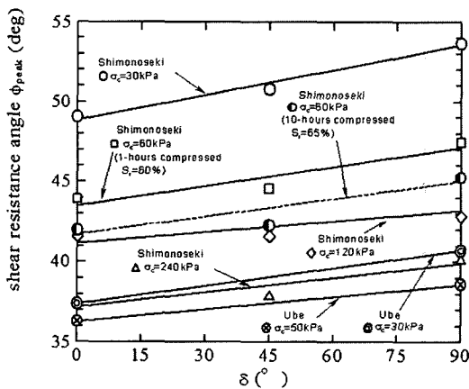
Fig. 10. Relationship between shear resistance angles at peak shear and \delta
