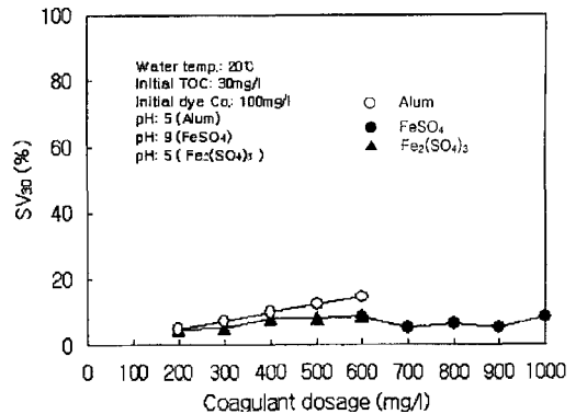
Fig. 4. SV 30 with various coagulant dosage using several coagulants(DB56).
