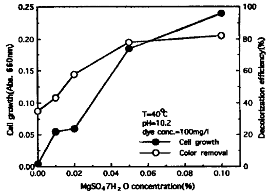
Fig. 5. Cell growth and color removal with MgSO 4 ·7H 2 O concentration.
