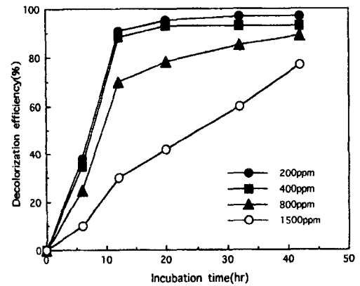
Fig. 8. Effect of dye concentration on the decolorization of strains, RBK1 (culture conditions: temp. 30°C, initial pH 7.0, shaking 180rpm).
