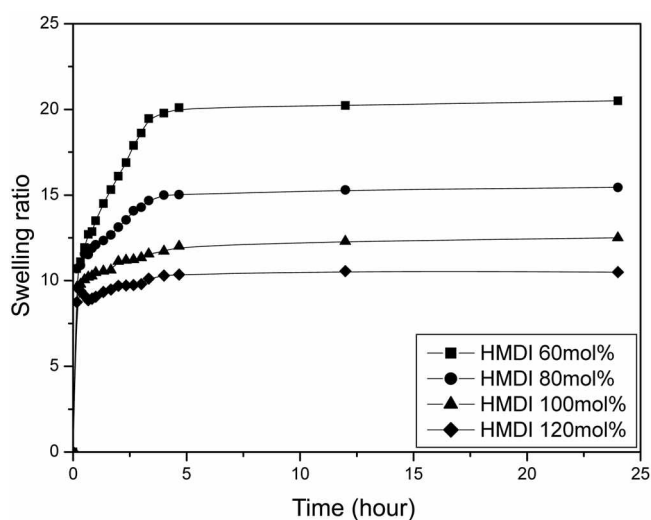
Figure 3. Typical swelling curves of gels in pure water at 25 °C.
