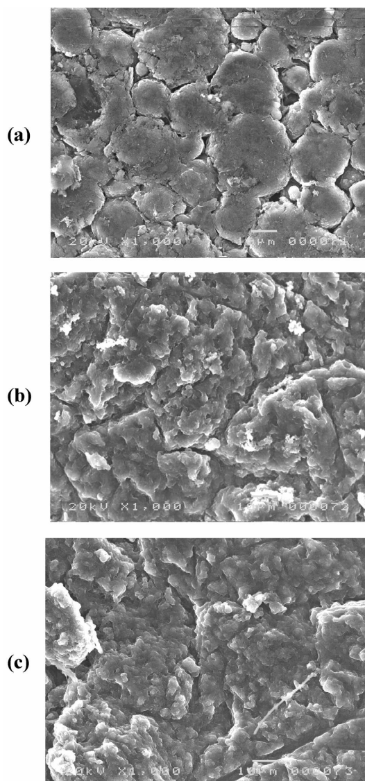
Figure 4. SEM images of the KMFC electrode surface in (a) bare, (b) 1 M \text{LiPF}_6/\text{pure PC} , and (c) 1 M \text{LiPF}_6/\text{PC} : \text{DEC} (4 : 1, \text{v/v}) .
