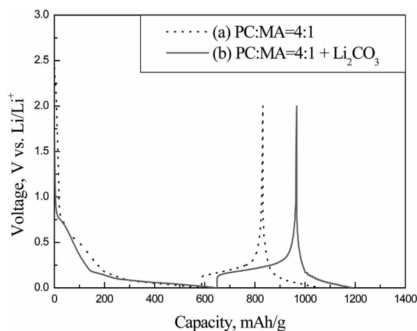
Figure 2. Voltage-capacity profiles of the KMFC electrode in (a) 1 M \text{LiPF}_6/\text{PC} : \text{MA} (4 : 1, v/v) and (b) 1 M \text{LiPF}_6/\text{PC} : \text{MA} (4 : 1, v/v) + \text{Li}_2\text{CO}_3 at a low rate of 0.5 \text{ mA}/\text{cm}^2 .
