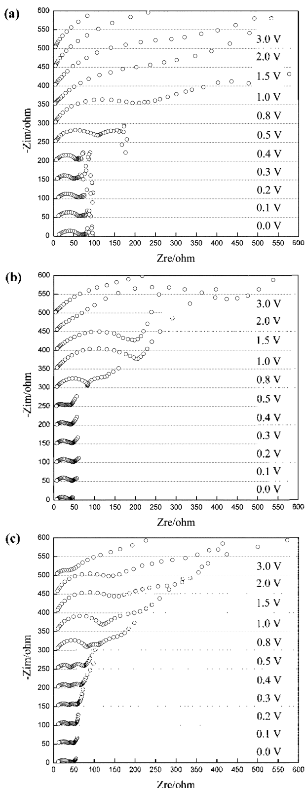
Figure 7. Impedance spectra of the KMFC electrode in (a) 1 M \text{LiPF}_6 /pure PC, (b) 1 M \text{LiPF}_6 /PC : MA (4 : 1, v/v), and (c) 1 M \text{LiPF}_6 /PC : MA (4 : 1, v/v) + \text{Li}_2\text{CO}_3 .
