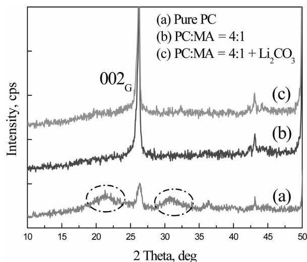
Figure 6. XRD patterns of the KMFC electrode after intercalation in (a) 1 M \text{LiPF}_6/\text{pure PC} , (b) 1 M \text{LiPF}_6/\text{PC} : \text{MA} (4 : 1, \text{v/v}) , and (c) 1 M \text{LiPF}_6/\text{PC} : \text{MA} (4 : 1, \text{v/v}) + \text{Li}_2\text{CO}_3 .
