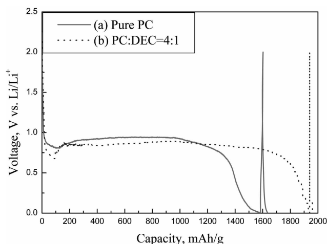
Figure 1. Voltage-capacity profiles of the KMFC electrode in (a) 1 M \text{LiPF}_6/\text{pure PC} and (b) 1 M \text{LiPF}_6/\text{PC} : \text{DEC} (4 : 1, v/v) at a low rate of 0.5 \text{ mA}/\text{cm}^2 .
