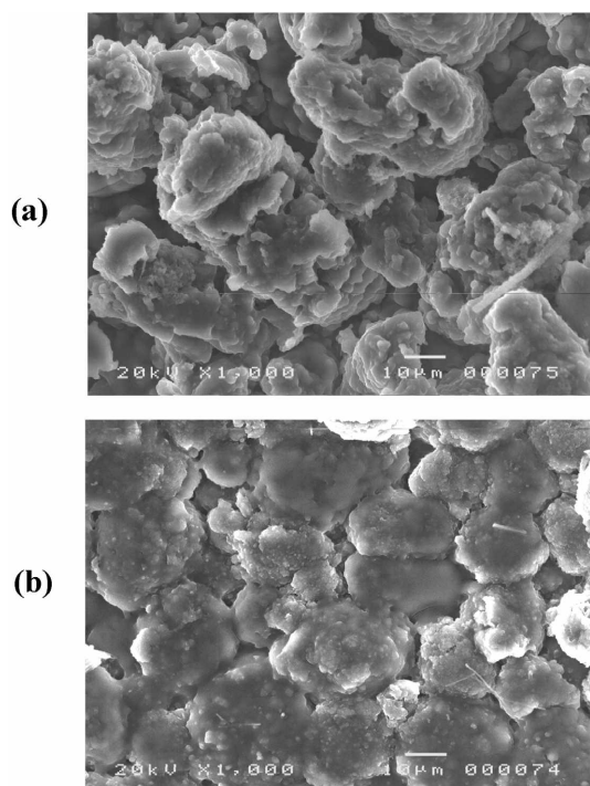
Figure 5. SEM images of the KMFC electrode surface in (a) 1 M \text{LiPF}_6/\text{PC} : \text{MA} (4 : 1, \text{v/v}) , and (b) 1 M \text{LiPF}_6/\text{PC} : \text{MA} (4 : 1, \text{v/v}) + \text{Li}_2\text{CO}_3 .
