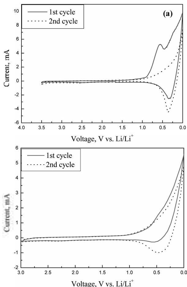
Figure 3. Cyclic voltammograms of the KMFC electrode in (a) 1 M \text{LiPF}_6/\text{PC} : \text{MA} (4 : 1, \text{v/v}) and (b) 1 M \text{LiPF}_6/\text{PC} : \text{MA} (4 : 1, \text{v/v}) + \text{Li}_2\text{CO}_3 .
