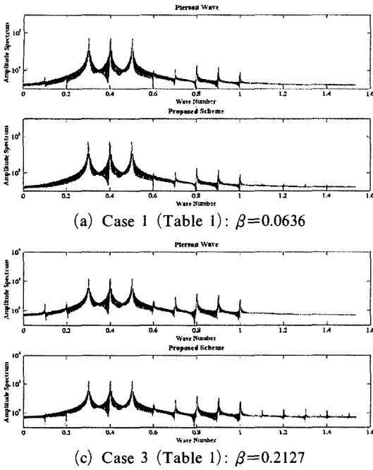
Fig. 4 Comparison of Wave Amplitude Spectra
