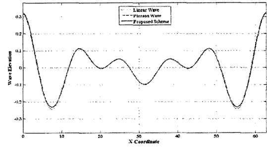
(b) Case 2 (Table 1): \beta=0.1345
