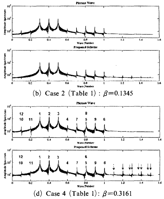
Fig. 4 Comparison of Wave Amplitude Spectra
