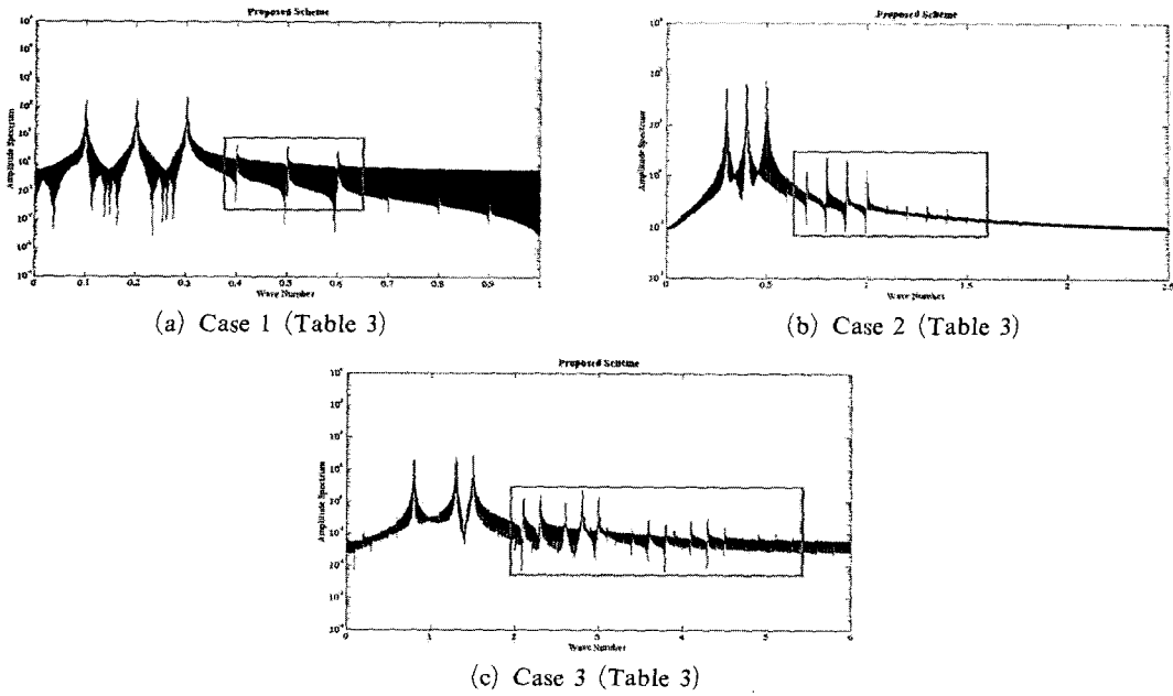
Fig. 6 Amplitude spectra (effect of wave numbers)
