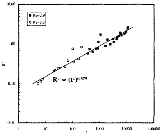
Fig. 13 Dimensionless bubble growth behavior for boiling flow at low Reynolds number
