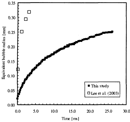
(a) Bubble radius comparison (dimensional scale)
