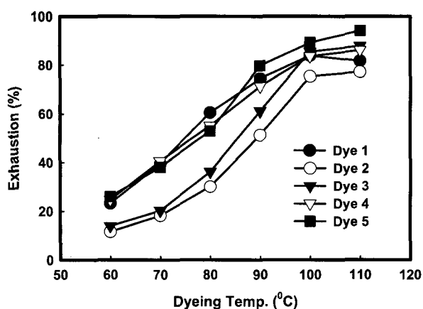
Fig. 5. Effect of application temperature on the extent of exhaustion.
