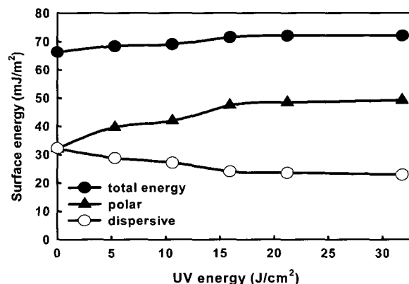
Fig. 5. Surface energy of UV-irradiated CA films.
