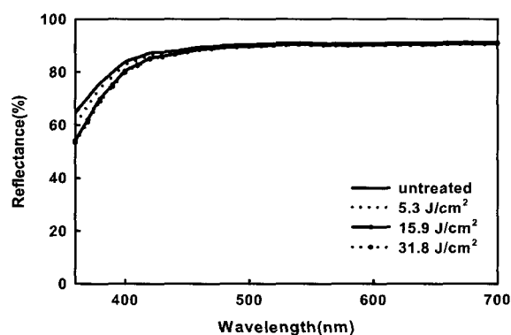
Fig. 1. Reflectance of UV-irradiated CA films.
