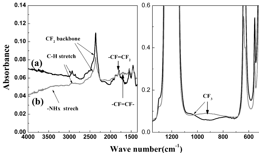
Fig 4. FT-IR spectra of PTFE irradiated in nitrogen gas (b) and unirradiated PTFE (a).
