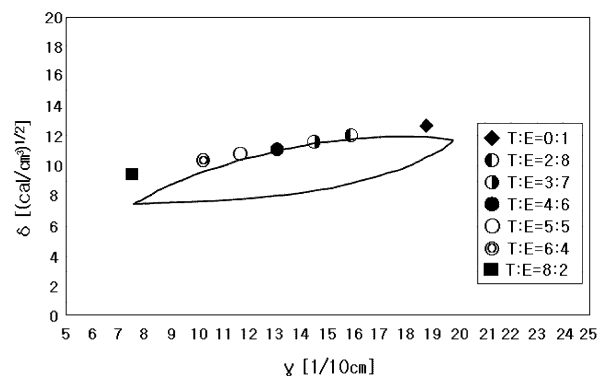
Fig. 1. Solubility of B79 resin plotted against solubility parameter ( \delta ) and hydrogen bonding index ( \gamma ).
