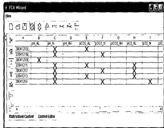
(그림 7) Derived One-valued context
