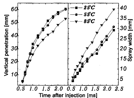
Fig. 6 Vertical penetration and spray width at different fuel temperatures
