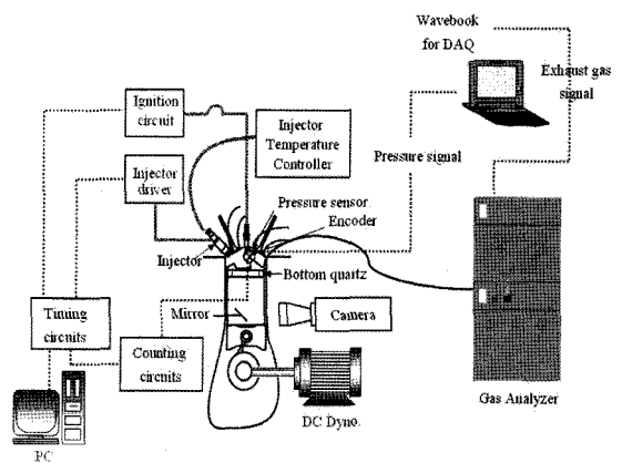
Fig. 2 Schematic diagram of engine setup
