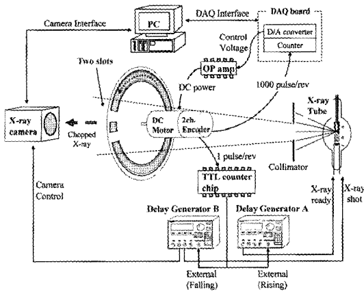
Fig. 4. Schematic diagram of Medical X-ray PIV system.
