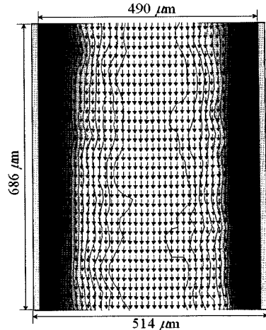
Fig. 3. Streamwise mean velocity field of whole blood flow in an opaque microchannel.
