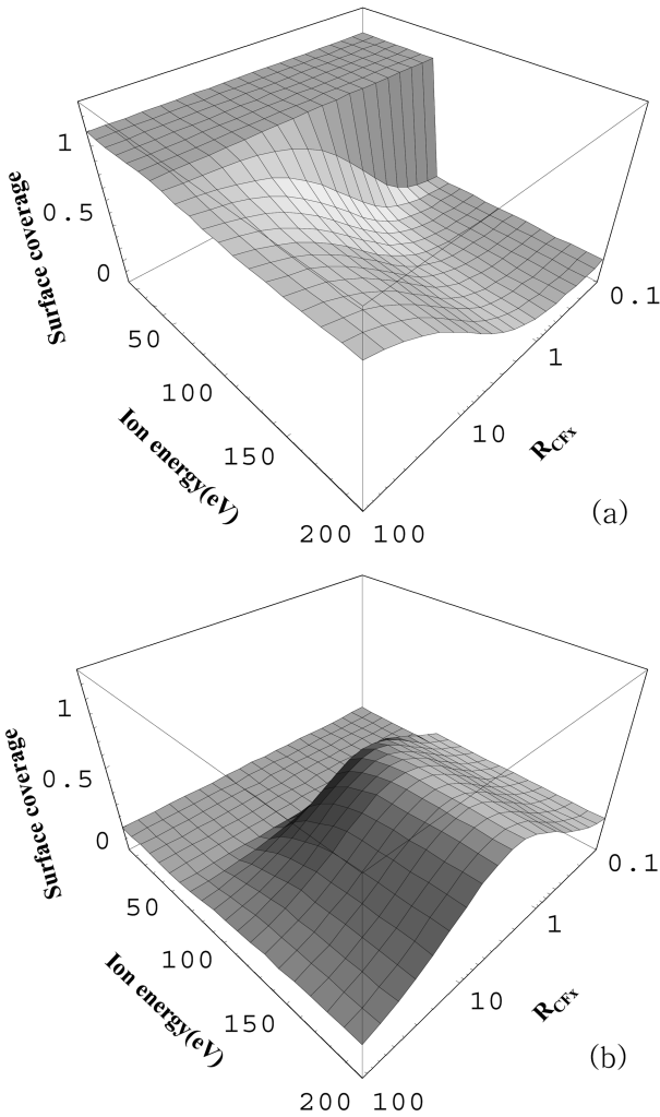
Fig. 5. Surface coverage as functions of R_{CFx} and ion energy. (a) polymer surface coverage, (b) CF_x surface coverage.
