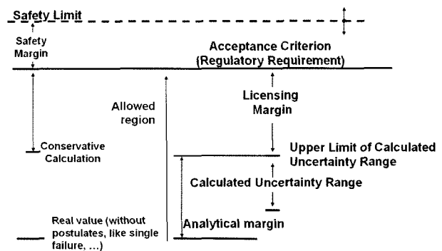
Fig. 2. Illustration of Safety Margins
