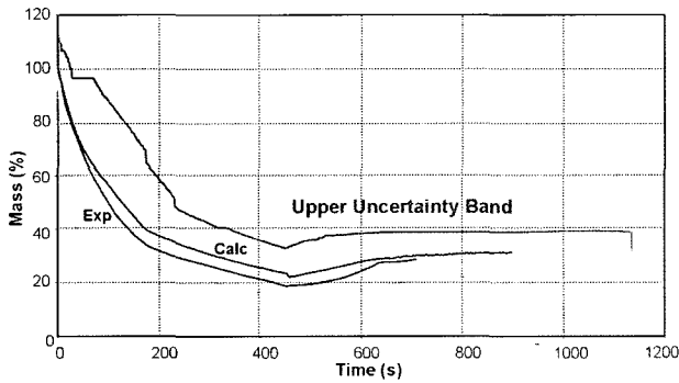
Fig. 8. Application of the CIAU to the UMS: Uncertainty Bands in Predicting Primary System Mass Inventory
