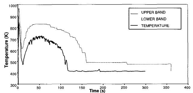
Fig. 6. Application of the CIAU to the Analysis of a Large Break LOCA in a Two-loop PWR: Rod Surface Temperature at 2/3 Core Height and Related Uncertainty Bands
