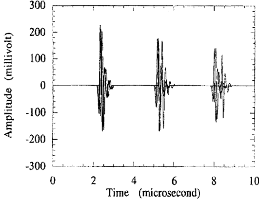
Fig. 2 Comparison of waveforms for three samples
