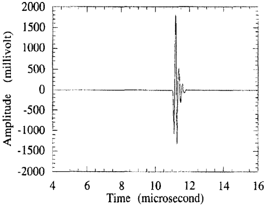
Fig. 3 Water path signal
