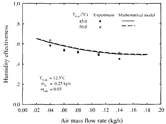
Fig. 22 Variation of the humidity effectiveness with air mass flow rate for different inlet-air temperatures at T_{w,in} = 12.5^\circ\text{C} , m_w = 0.25 kg/s
