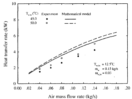
Fig. 15 Variation of the heat transfer rates with air mass flow rate for different inlet-air temperatures at T_{w,in}=12.5^{\circ}\text{C} , m_w=0.15 \text{ kg/s}
