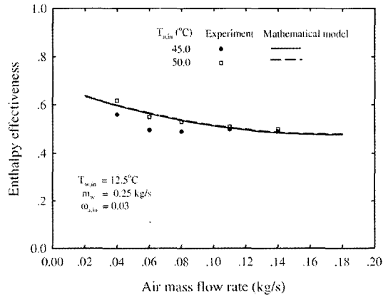
Fig. 21 Variation of the enthalpy effectiveness with air mass flow rate for different inlet-air temperatures at T_{w,in} = 12.5^\circ\text{C} , m_w = 0.25 kg/s
