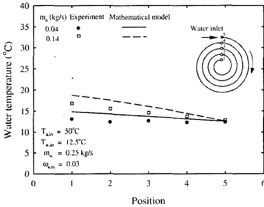
Fig. 5 Variation of water temperature with position along the spiral coil for difference air mass flow rates
