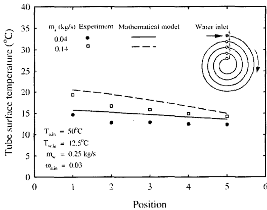
Fig. 6 Variation of tube surface temperature with position along the spiral coil for difference air mass flow rates
