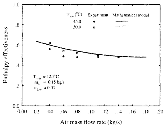
Fig. 19 Variation of the enthalpy effectiveness with air mass flow rate for different inlet-air temperatures at T_{w,in}=12.5^{\circ}\text{C} , m_w=0.15\text{ kg/s}
