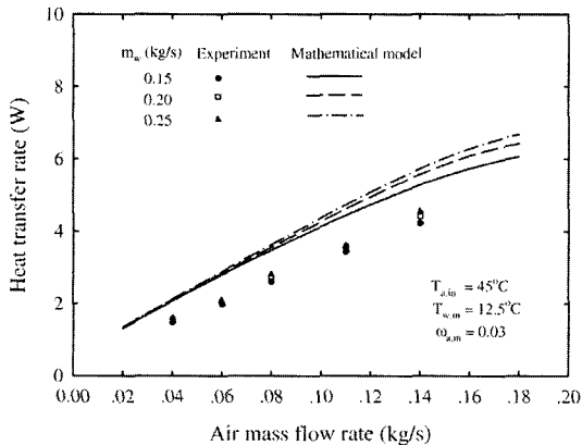
Fig. 17 Variation of the heat transfer rates with air mass flow rate for different water mass flow rates at T_{a,in}=45^{\circ}\text{C} , T_{w,in}=12.5^{\circ}\text{C}
