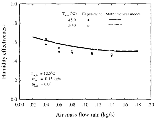
Fig. 20 Variation of the humidity effectiveness with air mass flow rate for different inlet-air temperatures at T_{w,in} = 12.5^\circ\text{C} , m_w = 0.15 kg/s
