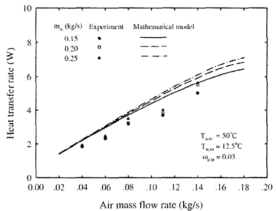
Fig. 18 Variation of the heat transfer rates with air mass flow rate for different water mass flow rates at T_{a,in}=50^{\circ}\text{C} , T_{w,in}=12.5^{\circ}\text{C}
