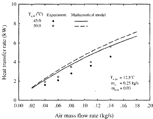
Fig. 16 Variation of the heat transfer rates with air mass flow rate for different inlet-air temperatures at T_{w,in}=12.5^{\circ}\text{C} , m_w=0.25\text{ kg/s}
