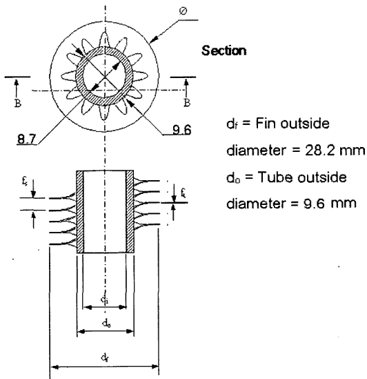
Fig. 3 Schematic diagram of crimped spiral fin
