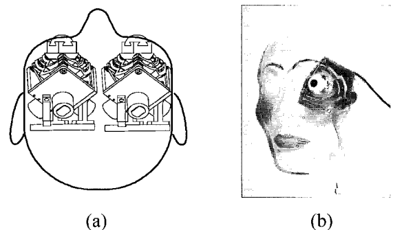
Fig. 3. The prototype of the 3-DOF anthropomorphic oculomotor simulator.
