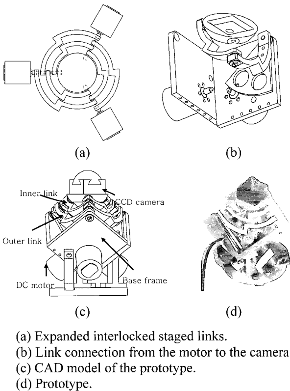
Fig. 2. The 3-DOF anthropomorphic oculomotor simulator.
