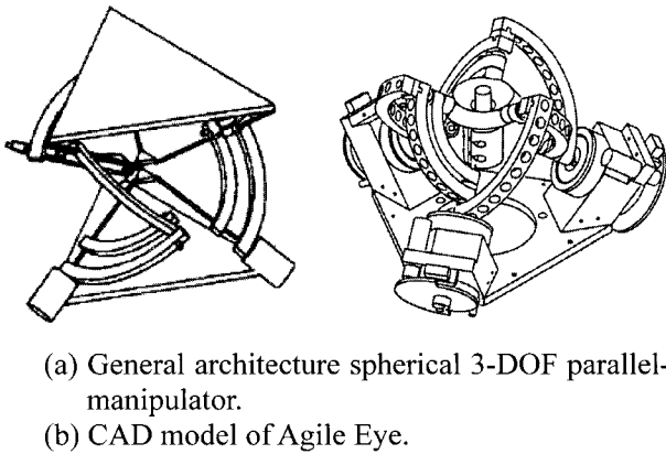
Fig. 1. Spherical 3-DOF parallel manipulator [9].
