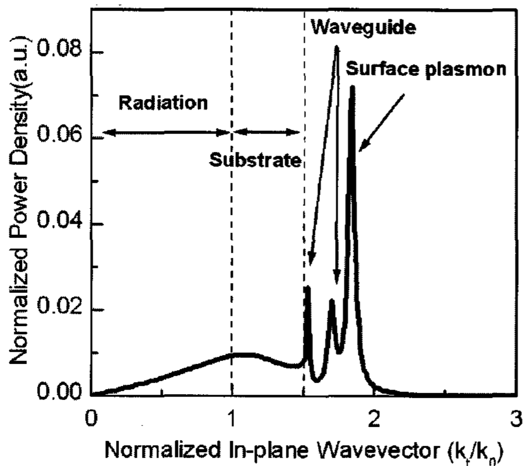
Fig. 2. Distribution of OLED emission into different modes.
