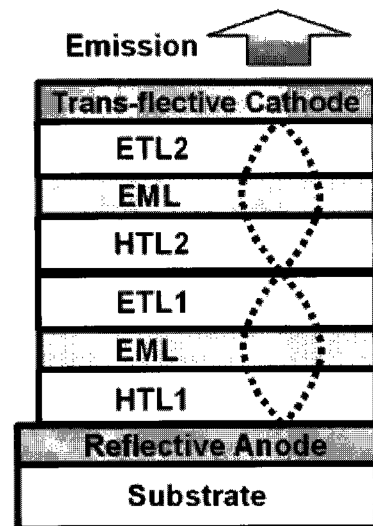
Fig. 7. Schematic structure of microcavity two-unit tandem OLED.
