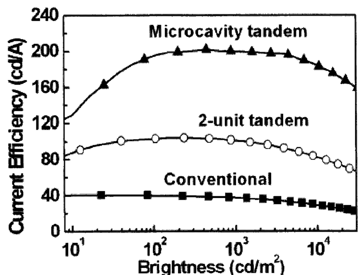
Fig. 8. cd/A efficiencies of various OLED structures.
