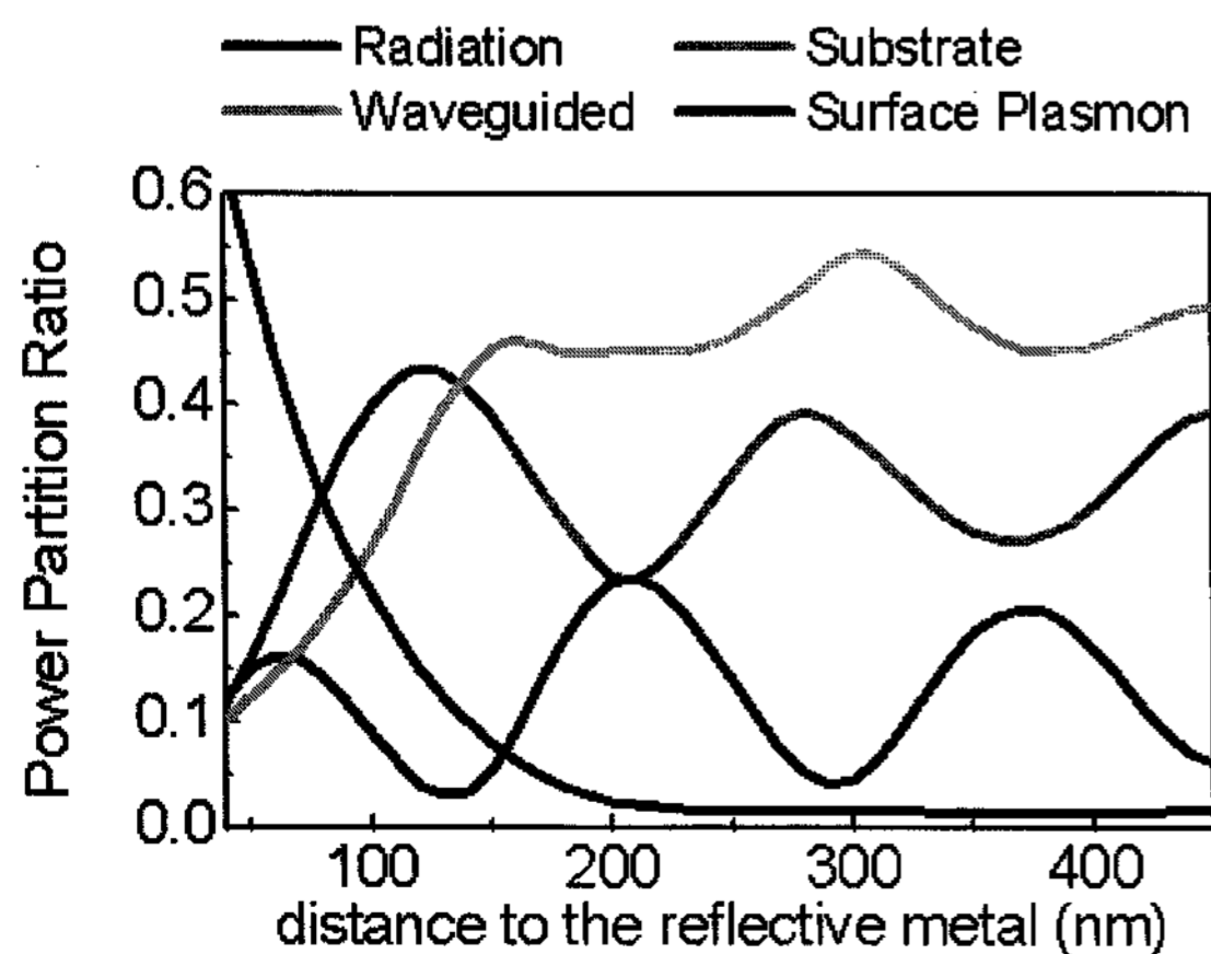
Fig. 6. Distribution of OLED internal radiation into different modes as a function of the emitter-to-reflector distance.
