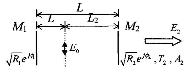
Fig. 3. Schematic structure of a microcavity OLED.
