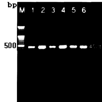
Fig. 9. Electrophoretic analysis of amplified products obtained by amplification PCR of cervical swab samples for Human Papilloma virus. Lane M: 100 bp DNA Ladder, Lane 1-6 : Human Papilloma virus(450 bp).
