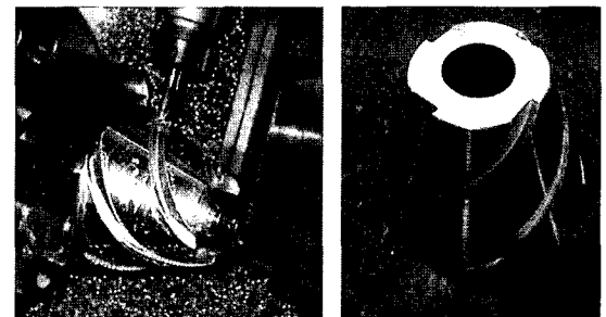
Fig. 9 5-axis NC machining using NC data generated by the E-POST
