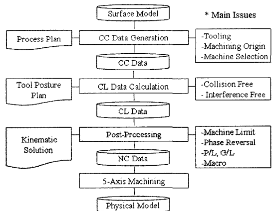
Fig. 1 Procedure for 5-axis NC machining
