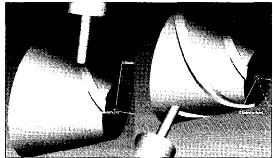
Fig. 8 Simulation of cutting using NC Data generated by the E-POST
