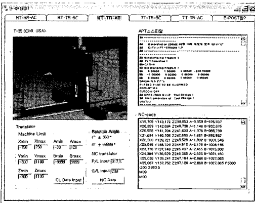
Fig. 6 Developed Post-Processor, E-POST
