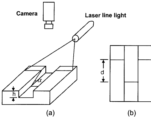
Fig. 2. Triangulation principle of slit ray projection.
