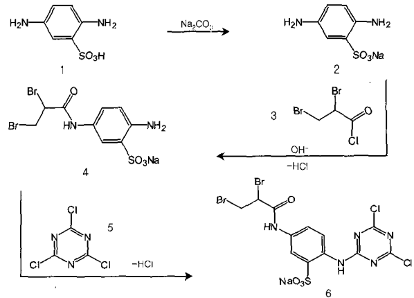
Fig. 1. Synthesis scheme of hetero-bi-functional reactive compound (Sodium-2-(2,3-dibromopropionylamino)-5-(4,6-dichloro-1,3,5-triazinylamino)-benzenesulfonate, DBDCBS).
