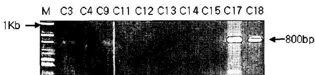
Fig. 3. Agarose gel showing products of blaSHV type from the two Escherichia coli strains. M; Standard ladder.
