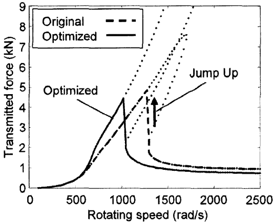
Fig. 10 Transmitted load for Case 5
