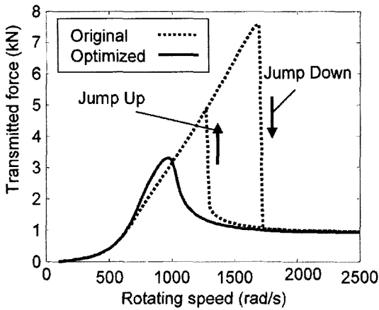
Fig. 9 Transmitted load for Cases 4 and 6
