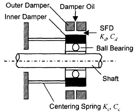
Fig. 1 Typical configuration of a squeeze film damper
