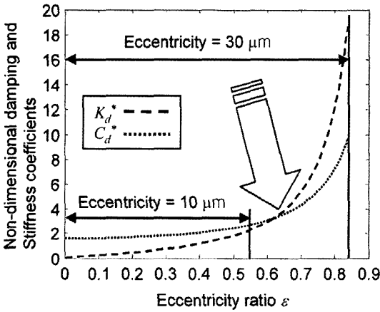
Fig. 2 Characteristics of stiffness and damping coefficients according to the variation of eccentricity ratio \varepsilon
