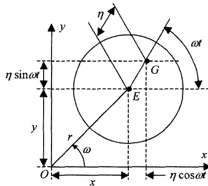
Fig. 5 Geometry of unbalance whirl at the disk
