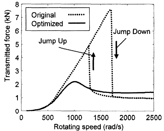
Fig. 11 Transmitted load for Case 7
