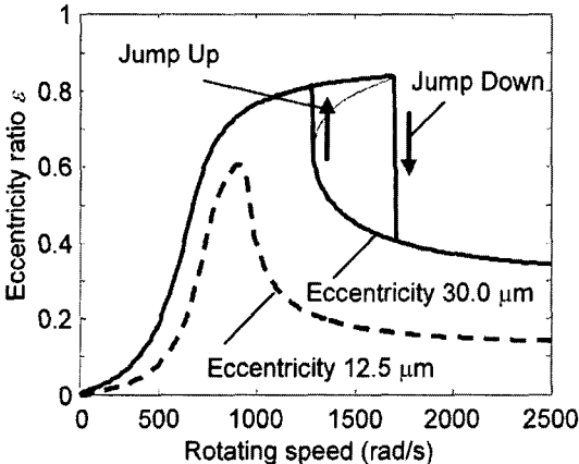
Fig. 3 Unbalanced response of a rotor system with SFD and single mass
