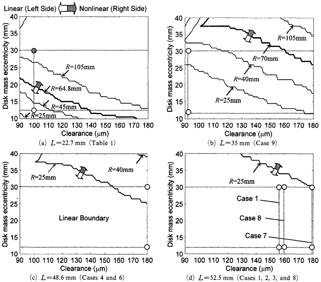
Fig. 15 Relation between linear and nonlinear responses for design parameters of SFD
