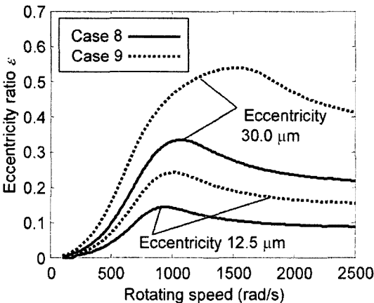
Fig. 14 Comparison eccentricity ratios of optimized SFDs between side constraints A and B
