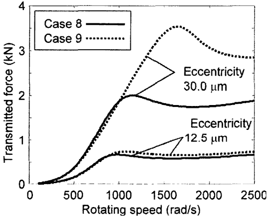
Fig. 13 Comparison transmitted load of optimized SFDs between side constraints A and B
