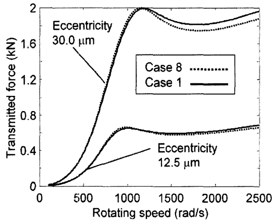
Fig. 12 Comparison transmitted load of optimized SFDs for nonlinear and linear responses
