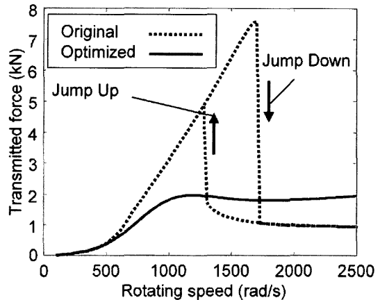
Fig. 8 Transmitted force for Cases 1, 2 and 3
