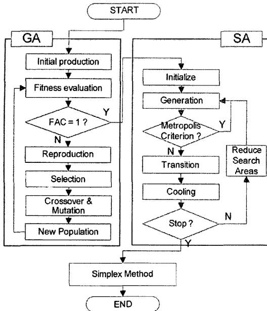
Fig. 6 Flow chart of HGASA
