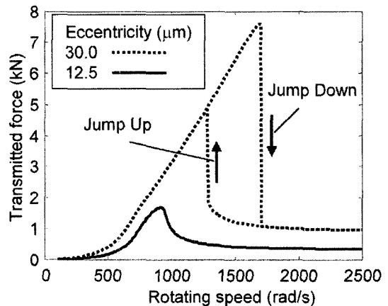
Fig. 7 Linear and nonlinear frequency responses according to disk mass eccentricity
