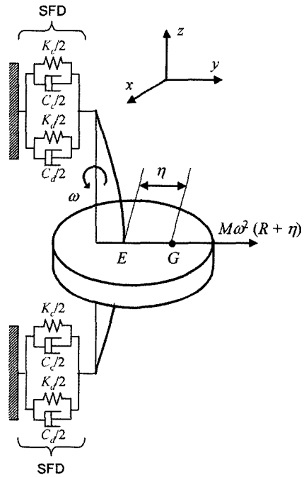
Fig. 4 Whirling of a flexible rotor system with squeeze film damper
