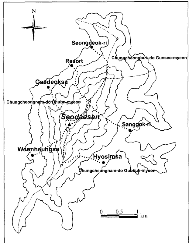
Fig. 1. A map of Seodaesan showing the investigated area and survey route.
