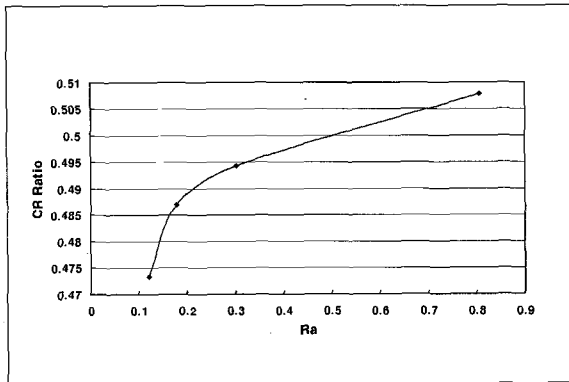
Contrast ratio = 0.468 + (0.0941 × Ra) + (0.0492 × Ra) 2 (R 2 = 0.81, F = 34.2)
