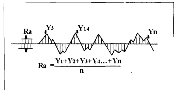
Figure 2. The overall roughness of the surface (Ra parameter) is defined as the arithmetical average value of all absolute distances of the roughness profile from the centerline within the measuring length.
