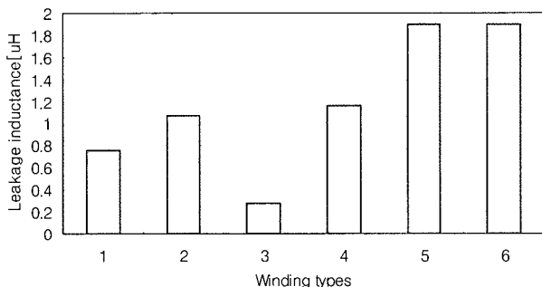
Fig. 11. Leakage inductance to winding types
