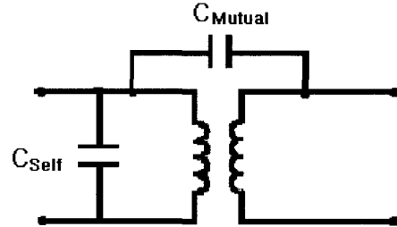
Fig. 3. Self-capacitance and mutual capacitance of EI28 models
