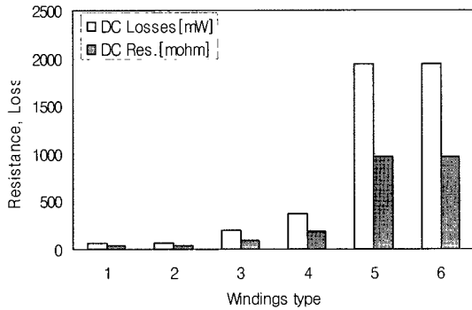
Fig. 9. DC loss and resistance for winding types
