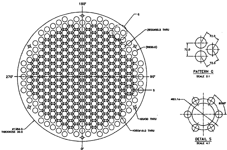
Fig. 2 Perforated plate
