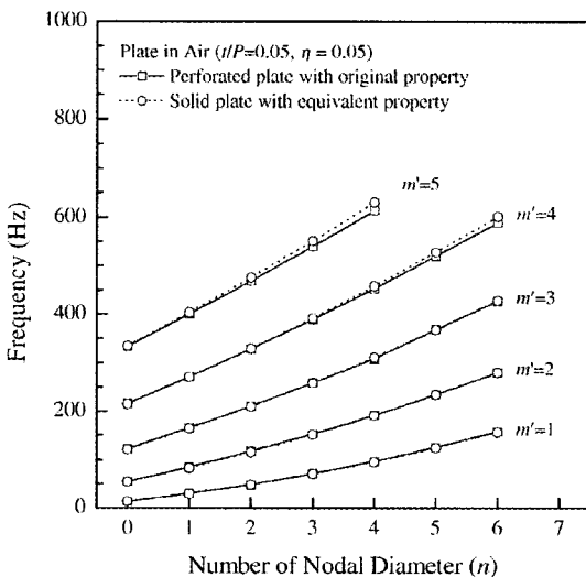
Fig. 17 Comparison of frequencies between perforated plate with original property and solid plate with equivalent property
