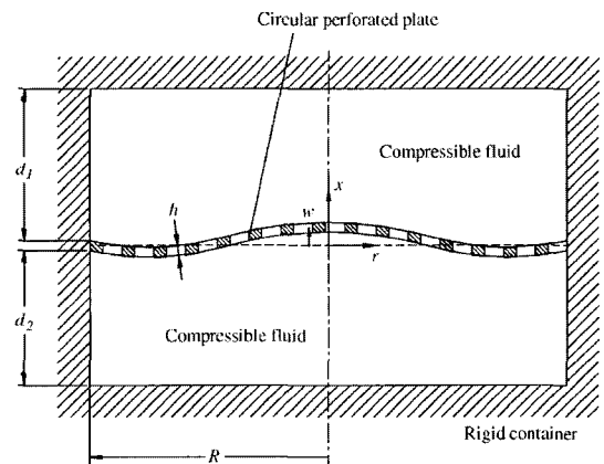
Fig. 1 Plate submerged in fluid
