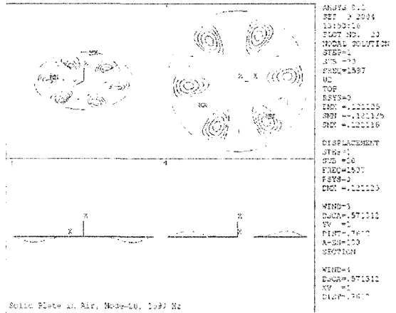
Fig. 8 Typical mode shapes of solid plate (Cont'd)
