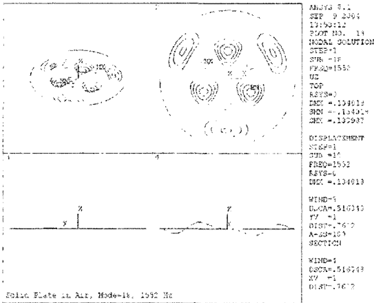
Fig. 8 Typical mode shapes of solid plate (Cont'd)
