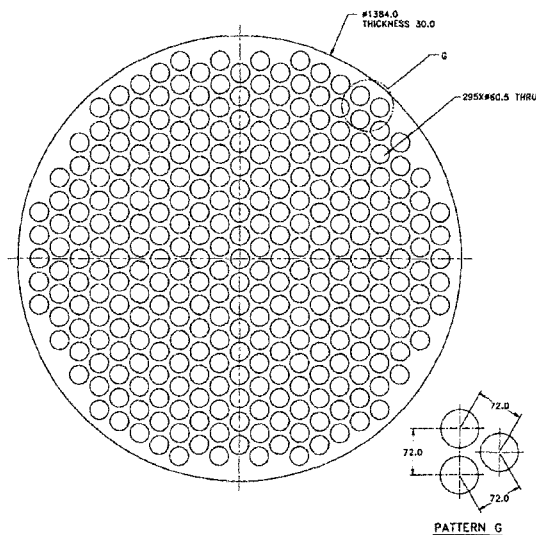
Fig. 14 Perforated plate with a triangular penetration pattern
