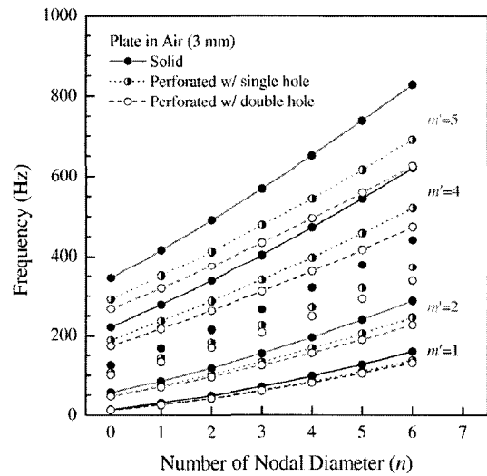
Fig. 6 Frequency comparisons between solid and perforated plates in air
