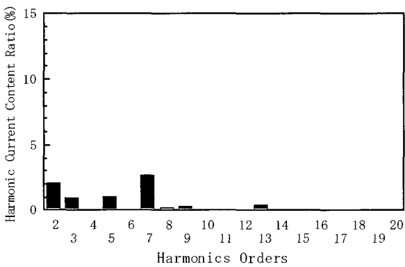
Fig. 15 Spectrum analysis of input current of improved active PFC converter in case of 46% dutyfactor
