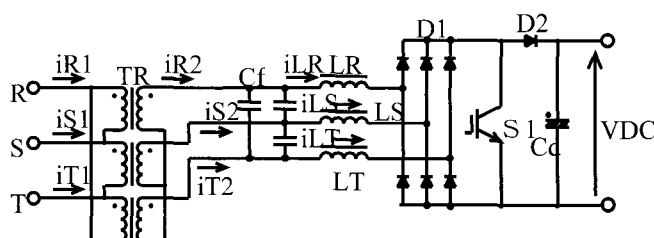
Fig. 1 Conventional circuit configuration of one-switch boost type active three phase PFC converter
