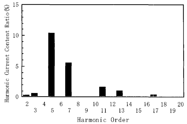
Fig. 3 Spectrum analysis of input current one-switch type three phase PFC active converter
