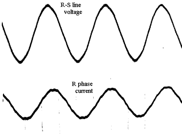
Fig. 13 Input voltage and current waveforms of improved type three-phase PFC active converter. (50V/div. 2.5A/div. 5.0mS/div.)
