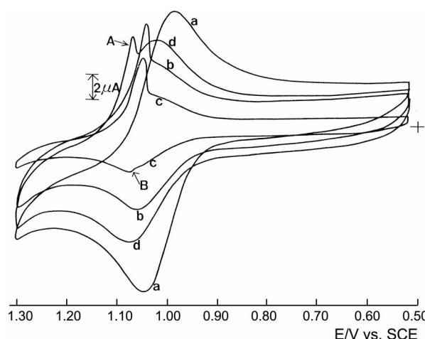
Figure 1. Cyclic voltammograms of 1.0 \text{ mM} \text{Ru}(\text{bpy})_3^{2+} in 100 \text{ mM} \text{H}_2\text{SO}_4 with and without SDS at 25.0 \pm 0.2 \text{ }^\circ\text{C} . Scan rate = 100 \text{ mV/s} except for [\text{SDS}] = 4.5 \text{ mM} ( 20 \text{ mV/s} ). (a) [\text{SDS}] = 0 \text{ mM} ; (b) [\text{SDS}] = 3.5 \text{ mM} ; (c) [\text{SDS}] = 4.5 \text{ mM} ; (d) [\text{SDS}] = 7.0 \text{ mM} .
