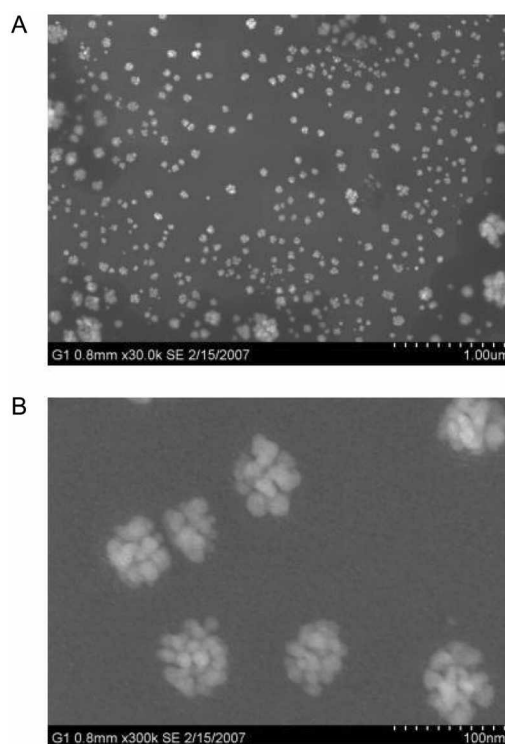
Figure 2. FE-SEM images of the GC electrode surface. The same polymer-modified electrode for Figure 1 was used. The electrode was initially immersed in a 0.5 mM \text{HAuCl}_4 solution for 20 min and the incorporated \text{AuCl}_4^- ions were reduced by the cyclic voltammetric scanning, as shown in Figure 1.
