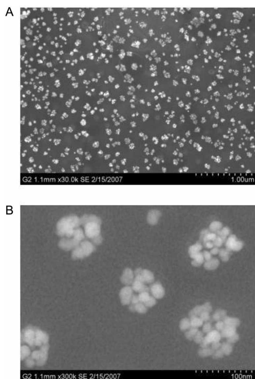
Figure 3. FE-SEM images of the GC electrode surface. The same polymer-modified electrode for Figure 1 was used. The electrode was initially immersed in a 0.5 mM \text{HAuCl}_4 solution for 50 min and the incorporated \text{AuCl}_4^- ions were reduced by the cyclic voltammetric scanning, as shown in Figure 1.
