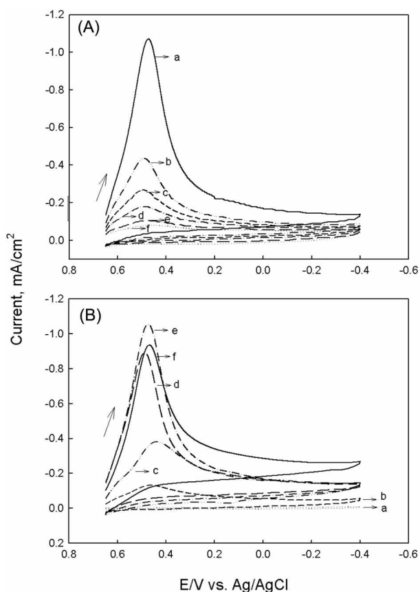
Figure 1. (A) Cyclic voltammograms in a pure supporting electrolyte. A GC electrode coated with 8 \mu\text{L} of a 1.5 mg/mL PVP and 0.36 mg/mL 1,12-dibromododecane mixture was used. The electrode, which had been previously immersed in a 0.5 mM \text{HAuCl}_4 solution for 50 min, was used. The first (a), 2nd (b), 3rd (c), 5th (d), 11th (e), and 20th (f) voltammograms after 5 min from the immersion of the introduction of the electrode into the cell solution were shown. (B) Cyclic voltammograms in a pure supporting electrolyte with the same GC electrode as Figure 1A. The electrode, which had been previously immersed in a 0.5 mM \text{HAuCl}_4 solution for 0 min (a), 10 min (b), 20 min (c), 30 min (d), 50 min (e), and 70 min (f), was used. Supporting electrolyte: 0.1 M \text{KCl} + 5.0 mM \text{HCl} . Scan rate: 50 mV/s.
