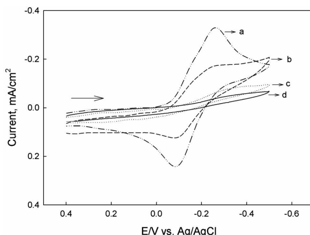
Figure 4. Cyclic voltammograms in a 3.0 mM \text{Ru}(\text{NH}_3)_6^{2+} with a GC electrode. The electrode was coated with 0 \mu\text{L} (a), 5 \mu\text{L} (b), 7 \mu\text{L} (c), and 8 \mu\text{L} aliquot (d) of 1.5 mg/mL PVP and 0.36 mg/mL 1,12-dibromododecane mixture. The other conditions were the same as shown in Figure 1.
