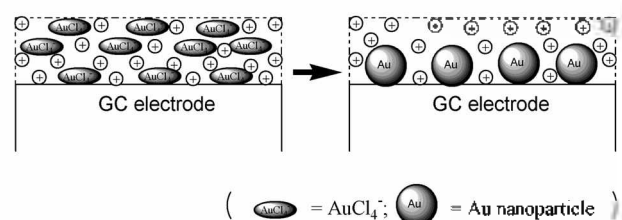
B. Formation of gold nanoparticles by the electro-reduction of \text{AuCl}_4^- ions
