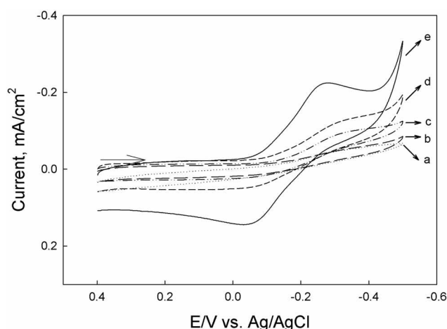
Figure 5. Cyclic voltammograms in a 3.0 mM \text{Ru}(\text{NH}_3)_6^{2+} with a GC electrode coated with an aliquot of 8 \mu\text{L} of 1.5 mg/mL PVP and 0.36 mg/mL 1,12-dibromododecane mixture coated. The conditions used for the nanoparticle formation: the electrode was initially immersed in a 0.5 mM \text{HAuCl}_4 solution for 0 min (a), 5 min (b), 10 min (c), 20 min (d), and 50 min (e) to allow the incorporated \text{AuCl}_4^- ions to be reduced by the potential step to 0.1 V from 0.8 V for 600 s in a pure 0.1 M KCl + 5 mM HCl supporting electrolyte. The other conditions were the same as shown in Figure 1.
