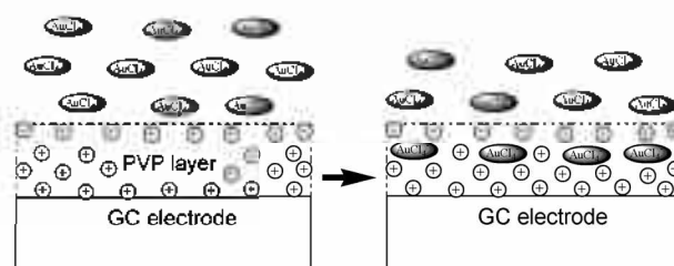
A. Incorporation of \text{AuCl}_4^- ions
