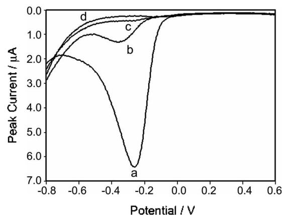
Figure 2. Differential pulse voltammograms for the acetylene black electrode in the presence (a) 3.0 \times 10^{-7} \text{ mol L}^{-1} hemoglobin and 4.0 \times 10^{-4} \text{ mol L}^{-1} SDS; (b) 3.0 \times 10^{-7} \text{ mol L}^{-1} hemoglobin; (c) 4.0 \times 10^{-4} \text{ mol L}^{-1} SDS and (d) phosphate buffer.
