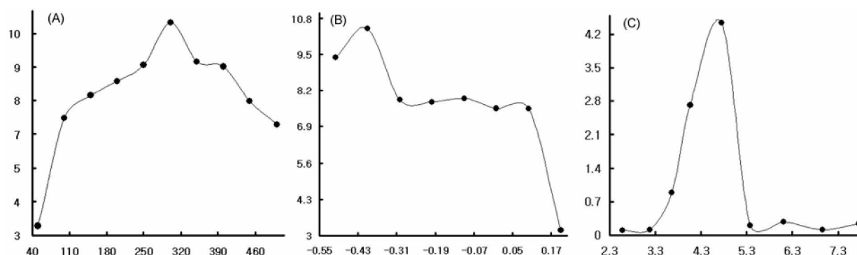
Figure 2. (A): Current response in SWSV accumulation times of 50, 100, 150, 200, 250, 300, 350, 400, 450 and 500 s. (B): Accumulation potentials of -0.5 , -0.4 , -0.3 , -0.2 , 0 , 0.1 and 0.2 V. (C): Electrolyte hydrogen ionic strength for 2.58, 3.18, 3.66, 4.75, 5.37, 6.11, 6.96 and 7.76 pH in 0.65 \text{ mgL}^{-1} glycine spike. Other experimental conditions used are the same as those in Fig. 3.
