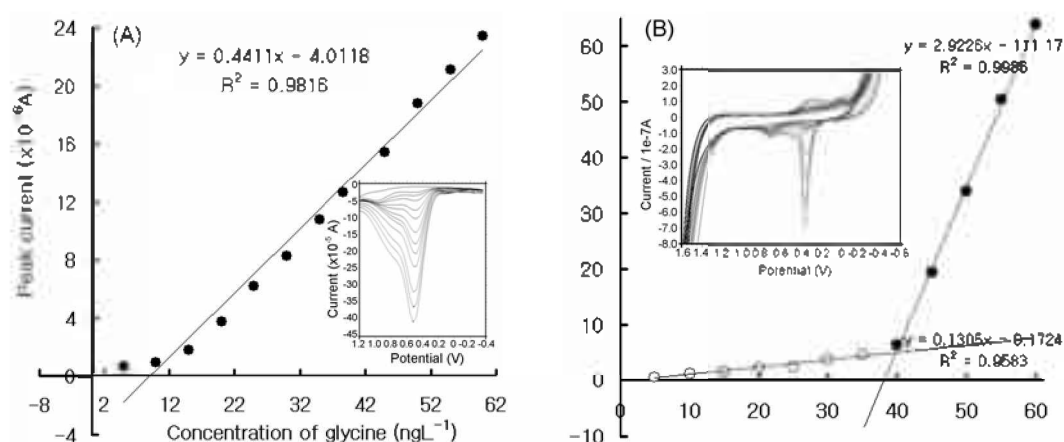
Figure 3. (A): SWSV and (B): CV working ranges of 5-, 10-, 15-, 20-, 25-, 30-, 35-, 40-, 45-, 50-, 55- and 60 \text{ ngL}^{-1} glycine in a 0.1 \text{ M} ammonium phosphate solution. SWSV: An amplitude of 0.2 \text{ V} , frequency of 500 \text{ Hz} , accumulation potential of -0.4 \text{ V} and accumulation time of 300 \text{ s} were used with a pH of 4.75 . CV: An initial potential of -0.6 \text{ V} , switching potential of 1.6 \text{ V} and scan rate of 0.5 \text{ V/s} were used.
