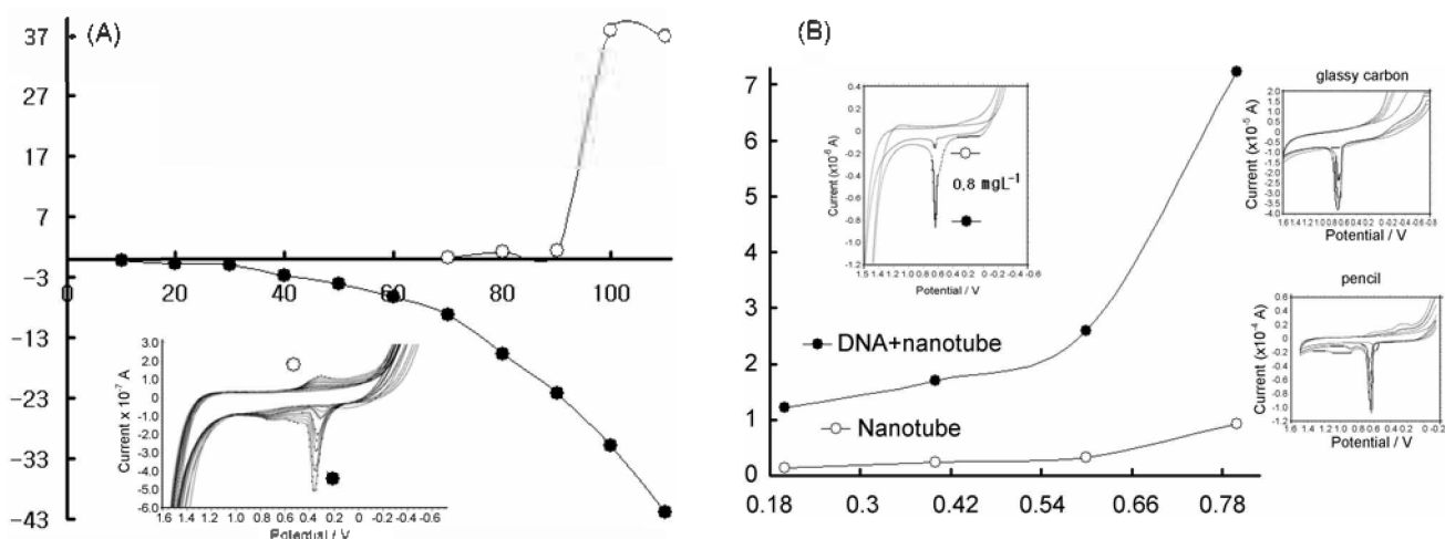
Figure 1. (A): Cyclic voltammetry for DNAPE, various concentrations of 10 -, 20 -, 30 -, 40 -, 50 -, 60 -, 70 -, 80 -, 90 -, 100 - and 110 \text{ µgL}^{-1} glycine spike. (B): Comparison of the carbon nanotube ( -\square- ) and DNAPE ( -\bullet- ) electrodes in glycine concentrations of 0.2 , 0.4 , 0.6 and 0.8 \text{ mgL}^{-1} using cyclic voltammetry (inner CV: 0.8 \text{ mgL}^{-1} ) in a 0.1 \text{ M} ammonium phosphate solution ( \text{pH } 4.5 ) with a scan rate of 100 \text{ mVs}^{-1} .
