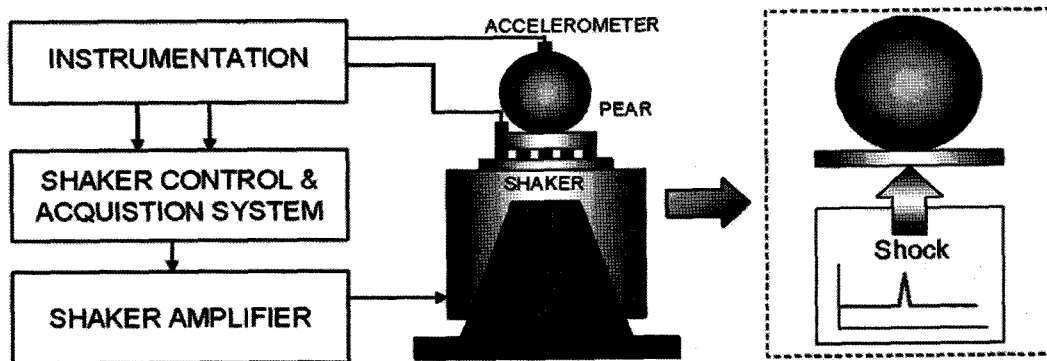
Fig. 1 Schematic diagram of the shock test apparatus for the pears.
