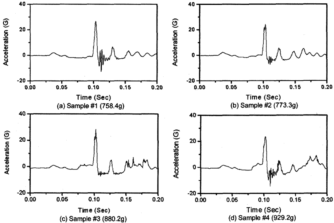
Fig. 4 Shock acceleration of the pears in shock profile input according to the mass.
