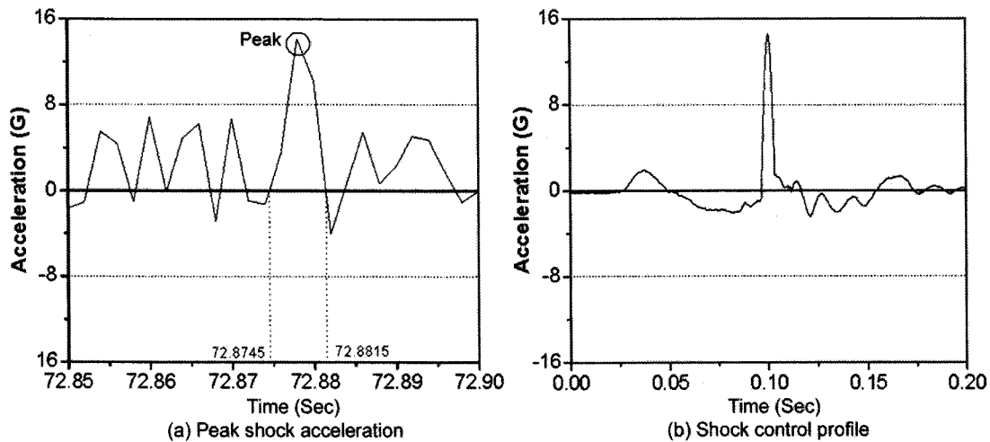
Fig. 3 Extended peak shock acceleration section in non-paved road and shock control profile.
