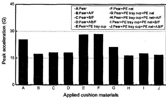
Fig. 5 Shock accelerations of the pears by cushion packaging materials in shock profile input.
