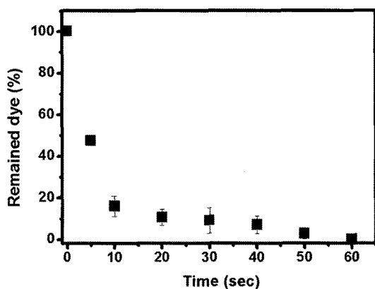
Figure 5. Release profile of dye-loaded PEtOz-PCL micelle from 6.5 bilayer thin film after dipping in aqueous solution at pH 5.6.
