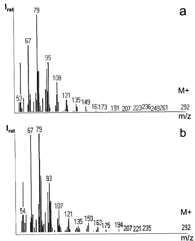
Fig. 1. GC/EI-MS full scan spectra of the methyl esters of (a) α-linolenic acid (ALA/18:3n-3) and (b) γ-Linolenic acid (GLA/18:3n-6).
