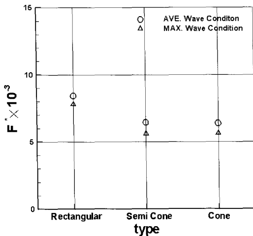
Fig. 3 Force at Inlet in Various Wave Condition.
