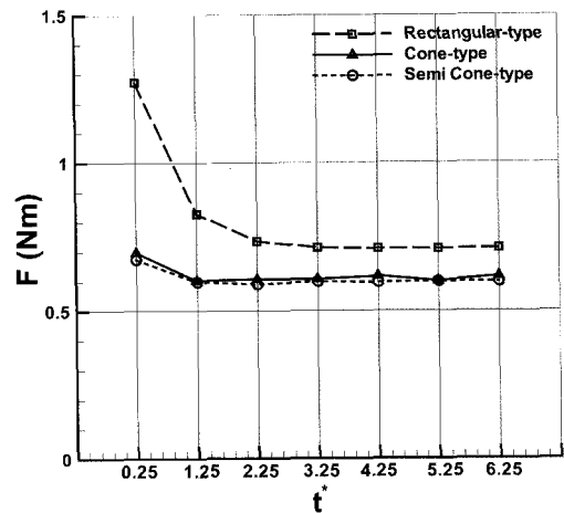
Fig. 4 Force Variation at Inlet of Air Chamber per Period
