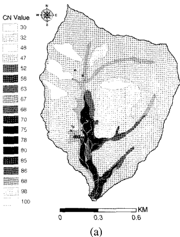
Fig. 5. SCS-CN distribution from (a) 1:5,000 soil and QuickBird land use, (b) 1:25,000 soil and land use, (c) 1:50,000 soil and land use.
