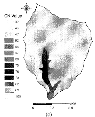
Fig. 5. SCS-CN distribution from (a) 1:5,000 soil and QuickBird land use, (b) 1:25,000 soil and land use, (c) 1:50,000 soil and land use.
