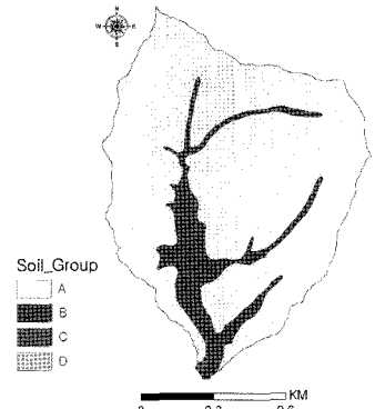
Fig. 4. Hydrologic soil group.
