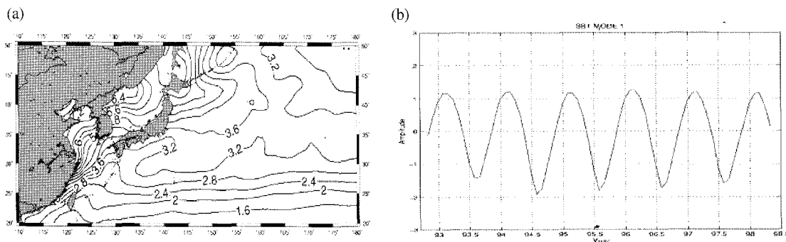
Fig. 5. (a) spatial field and (b) temporal amplitude of the first mode(94%) for SST.
