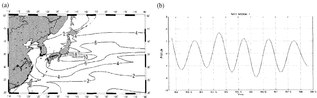
Fig. 4. (a) spatial field and (b) temporal amplitude of the first mode(40%) for SL.
