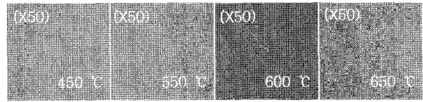
Fig. 5. Microscopic images of the InGaN buffer layers.
