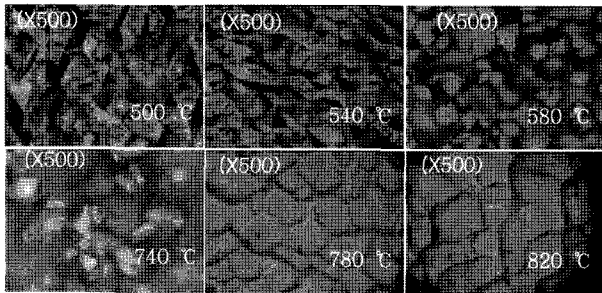
Fig. 8. Microscopic images of the HT-GaN grown on LT-GaN buffer layers.
