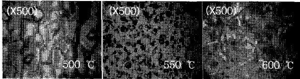
Fig. 3. Microscopic images of the HT (high temperature)-GaN grown on LT (low temperature)-AlN buffer layers.
