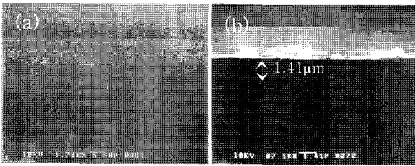
Fig. 9. SEM images of GaN buffer layer grown on r-plane sapphire substrate at 820°C. (a) plane-view (b) cross-section.
