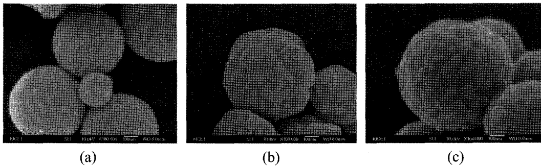
Fig. 5. FE-SEM images of \text{Ni}_{1-x}\text{Zn}_x\text{Fe}_2\text{O}_4 nanostructured particles; (a) before annealing, (b) x=0.4 and (c) x=0.6 for annealed powder at 1273 K.
