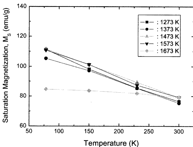
Fig. 9. Saturation magnetization of annealed \text{Ni}_{1-x}\text{Zn}_x\text{Fe}_2\text{O}_4 ( x=0.4 ) powders measured at different temperatures between 77 K and 300 K.
