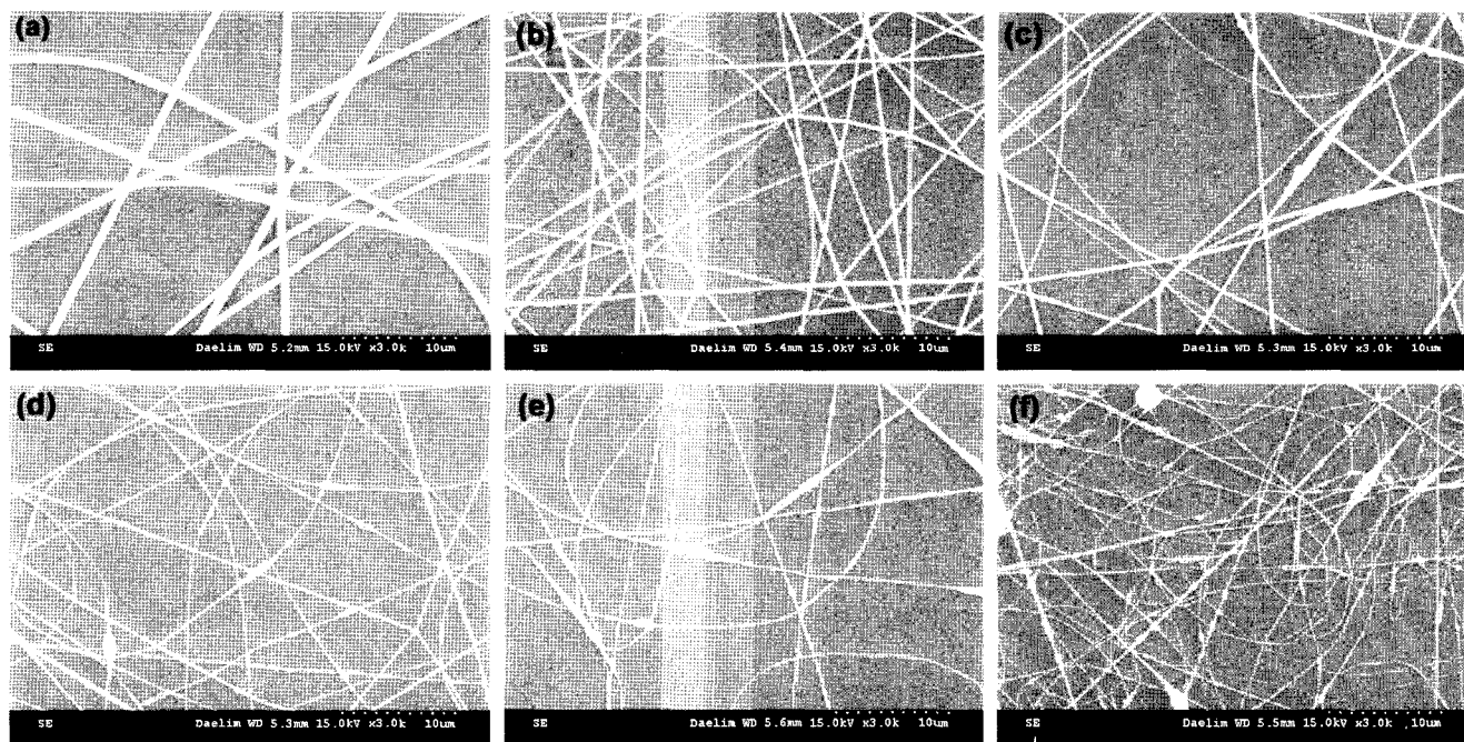
Fig. 1. SEM images of electrospun PAN/Fe 2 O 3 nanocomposite fibers as a function of the Fe 2 O 3 content; (a) 0%, (b) 1%, (c) 2%, (d) 5%, (e) 4%, and (f) 5%.
