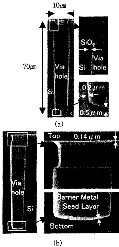
Fig. 6 Trough-hole produced by DRIE with scallop-shaped side wall: (a) as SiO_2 -film deposited (b) as barrier metal/seed layer deposited
