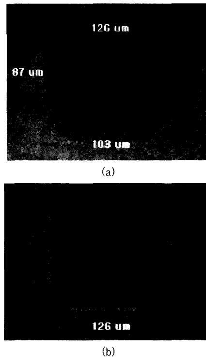
Fig. 4 U-groove machined by femtosecond laser (20Objective lens with 0.42 NA, 30-J pulse energy, scan speed of 500 m/s): (a) top view(500), (b) side view(500)
