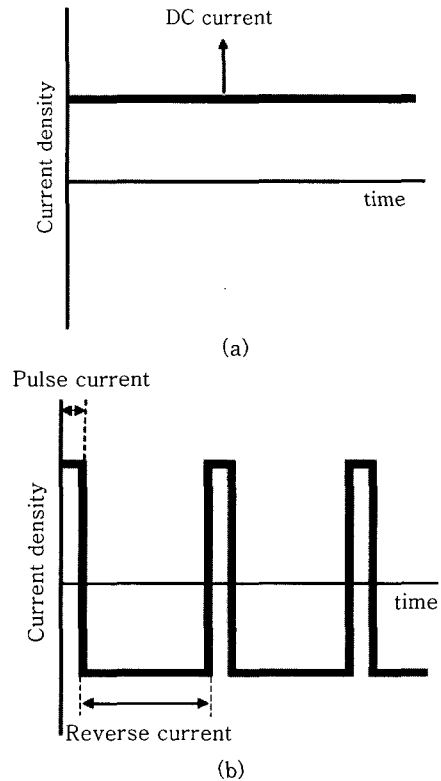
Fig. 7 Schematics of current mode: (a) DC current mode, (b) pulse-reverse current mode for this study
